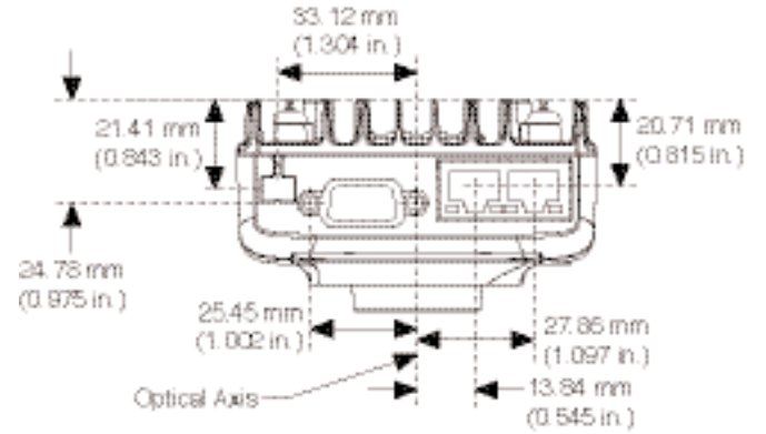
Figure 5. Camera Bottom
